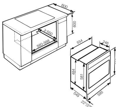
H 2261 B, 56 l cavity
