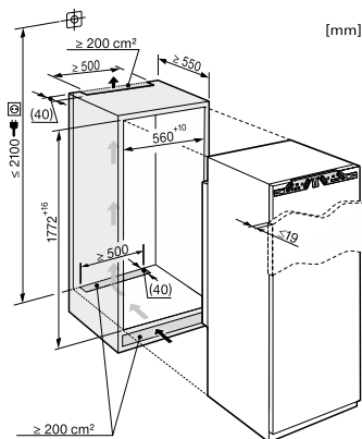
KS 37422 iD, FNS 37402 i
