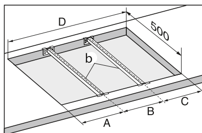
Worktop cut-out: 3 Appliances
