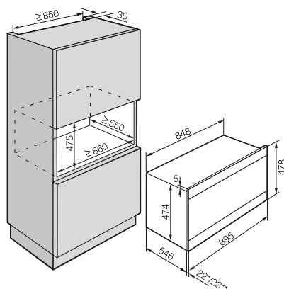
H 6890 BP, 90 l cavity
