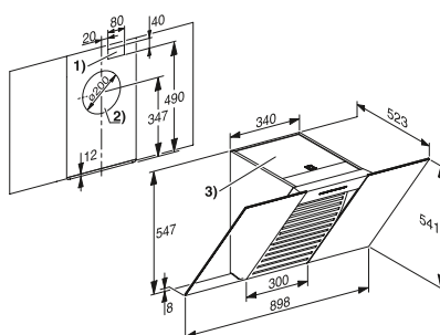
DA 6096 W - Wall mounted
