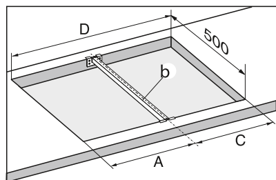
Worktop cut-out: 2 Appliances
