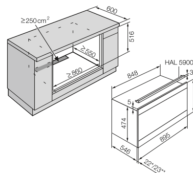
H 6890 BP, 90 l cavity
