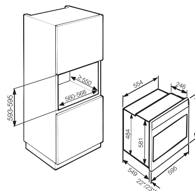
H 2261 B, 56 l cavity
