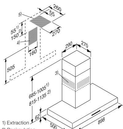
DA 429-6 - Wall mounted
