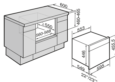
DG 6200, DG 6401, 38 l cavity
