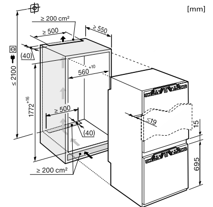
KFNS 37432 iD, KFNS 37452 iD
