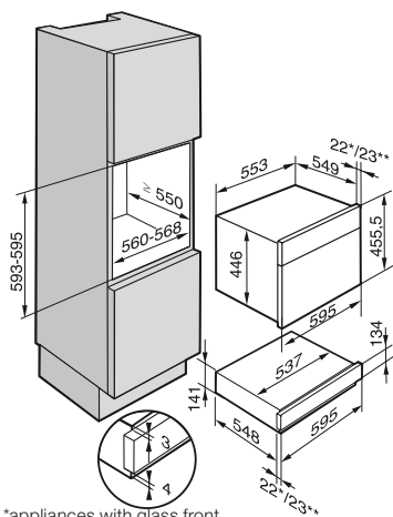
DG 6200, DG 6401, 38 l cavity
