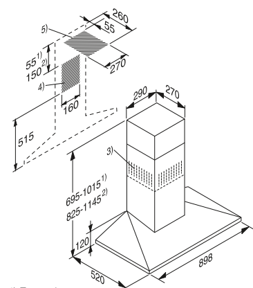
DA 399-6 - Wall mounted
