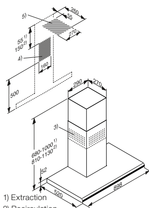
DA 6296 W - Wall mounted
